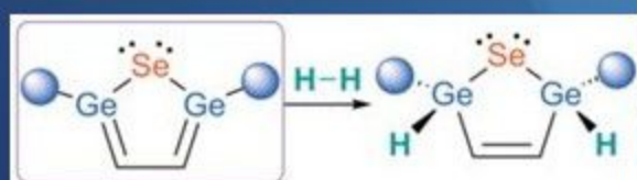
Dihydrogen Activation by a Digermaselenophene
