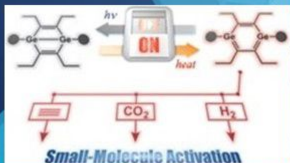
Dihydrogen Activation by a Digermaselenophene
