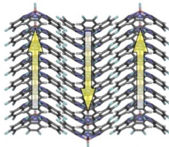
Centrosymmetric Structure
