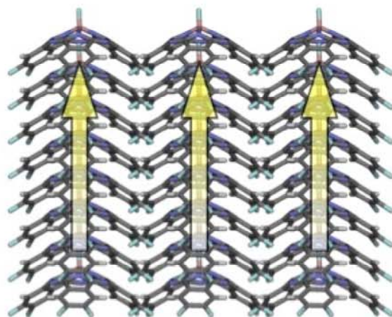
Non-centrosymmetric Structure
